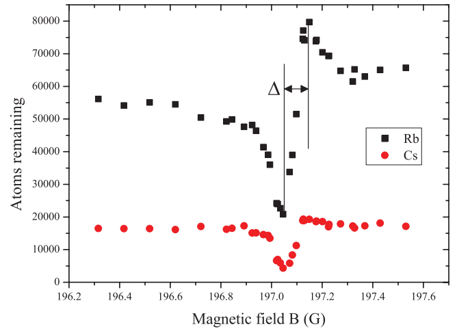
FIG. 3. (Color online) Example of a Feshbach resonance scan showing simultaneous loss for Rb and Cs near 197.06(5) G for a hold time of 200 ms. The maximum for the number of Rb atoms to the right of the resonance is attributed to the zero crossing for the interspecies scattering length. The difference in the positions of the minima and the maximum as indicated gives an estimate for the resonance width \Delta .
