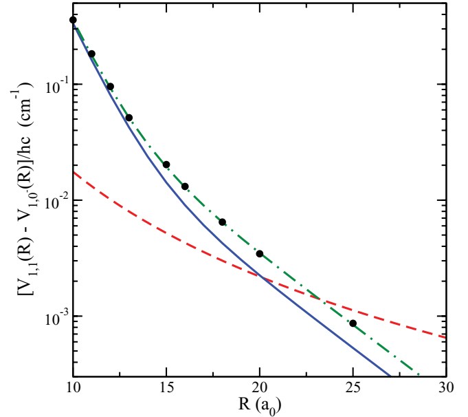
FIG. 7. (Color online) Study of the second-order spin-orbit interaction energy V_{1,1}(R) - V_{1,0}(R) as a function of internuclear separation R . The solid circles are the result of the ab initio RCI VB electronic structure calculation. The green dash-dotted line is a fit to the ab initio values using the functional form of Eq. (12). The blue line corresponds to the second-order spin-orbit interaction energy optimized to reproduce the location of the observed magnetic Feshbach resonances for A_{2SO}^{\text{long}} = -0.033 10. For comparison, the absolute value of the corresponding splitting due to the magnetic dipole-dipole interaction is shown by a red dashed line.
