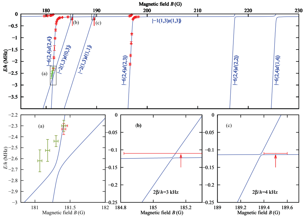
FIG. 5. (Color online) Weakly bound states of RbCs obtained by free-bound (red, dark-gray) and bound-free (green, gray) magnetic-field modulation spectroscopy, together with levels calculated for the final, fitted potentials (blue solid lines). All levels are shown relative to dissociation limit Rb |1,1\rangle + \text{Cs } |3,3\rangle at the given magnetic field value B . Avoided crossings between the least-bound state and the ramping n = -2 levels are shown as arrows. The smaller panels labeled (a), (b), and (c) refer to the areas on the larger panel marked by rectangles and the same labels. The quantity 2\beta is the minimum separation in energy between the two states.
