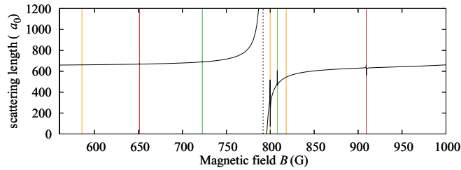
FIG. 11. (Color online) RbCs scattering length at the |1,1\rangle + |3,3\rangle threshold at fields above 560 G, calculated at E = 160 nK using the final fitted potential. Resonance positions are marked by vertical lines, with the value of M_F of the corresponding bound state indicated using the same color scheme as in Fig. 8.
