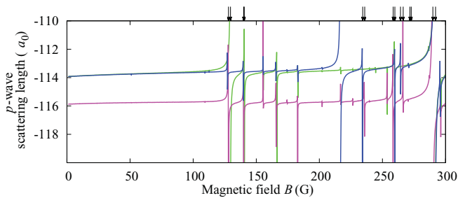
FIG. 9. (Color online) The p -wave scattering lengths at the |1,1\rangle + |3,3\rangle threshold for the three values of M allowed for p -wave scattering of Rb + Cs, calculated at E = 7 \mu K using the final fitted potentials. Results for M_F = 3, 4 , and 5 are shown as blue (dark gray), magenta (gray), and green (light gray), respectively. The observed positions of p -wave resonances are shown as arrows at the top of the graph.
