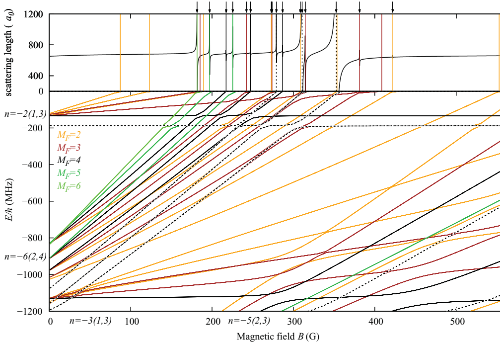
FIG. 8. (Color online) Weakly bound states of RbCs for M = 4 at fields up to 550 G, calculated using the final fitted potentials, together with the scattering length at the |1,1\rangle + |3,3\rangle threshold, calculated at E = 160 nK. Bound states are plotted in a color corresponding to their value of M_F , as shown on the figure. States arising from L = 2 ( d states) are shown as solid lines, and from L = 0 ( s states) are shown as dashed lines. The resonance positions are marked on the scattering length plot as vertical lines with the same color as the bound state that they arise from. The slanted text on the left-hand axis and below the bottom axis indicates which vibrational and hyperfine manifold the L = 2 bound states arise from. The least-bound state |-1(1,3)s(1,3)\rangle is within the thickness of the zero line on this scale. The observed positions of incoming s -wave resonances are shown as arrows above the plot.
