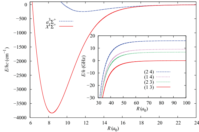
FIG. 1. (Color online) Molecular potential energy curves V_0(R) and V_1(R) for the singlet and triplet states of RbCs correlating with two separated ^2S_{1/2} ground-state atoms. The inset shows an expanded view of the long-range potentials separating to the four different hyperfine thresholds at zero field, labeled by (f_{^{87}\text{Rb}}, f_{^{133}\text{Cs}}) , but no longer by singlet or triplet.
