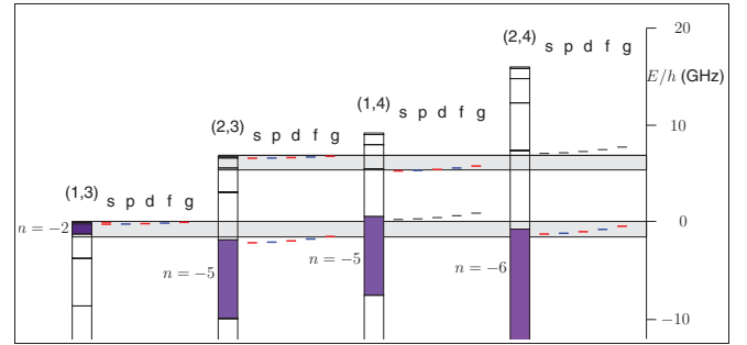
FIG. 2. (Color online) Thresholds for ^{87}\text{Rb}^{133}\text{Cs} and the bins (vertical boxes) below each threshold within which each vibrational state must lie for any value of the scattering length. The horizontal boxes, 1.5 GHz deep, show the energy range within which bound levels can cause resonances at the |1, 1\rangle + |3, 3\rangle and |2, -1\rangle + |3, 3\rangle thresholds at fields under 500 G. The vibrational bin for each hyperfine state that contains bound states that can cause resonances at the lowest threshold is colored. Selected levels are shown (short horizontal lines) as a function of L ( s, p, d, f, g for L = 0, 1, 2, 3, 4 , respectively) for the specific choice of scattering length that gives a least-bound state for L = 0 with 110(20) kHz below threshold. For fields below 500 G, only levels |n(f_{\text{Rb}}, f_{\text{Cs}})\rangle = |-2(1, 3)\rangle and |-6(2, 4)\rangle can cause resonances at the |1, 1\rangle + |3, 3\rangle threshold and only levels |-4(1, 4)\rangle and |-2(2, 3)\rangle can cause resonances at the |2, -1\rangle + |3, 3\rangle threshold.
