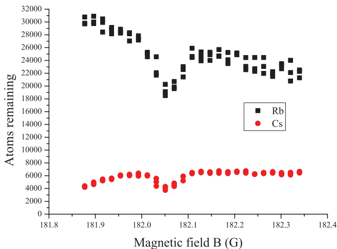
FIG. 4. (Color online) Measurement of the binding energy of the Feshbach molecules. This is an example of a field modulation free-bound resonance scan showing simultaneous loss for Rb and Cs for a hold time of 900 ms. The modulation frequency is held fixed at f_m = 330 kHz.
