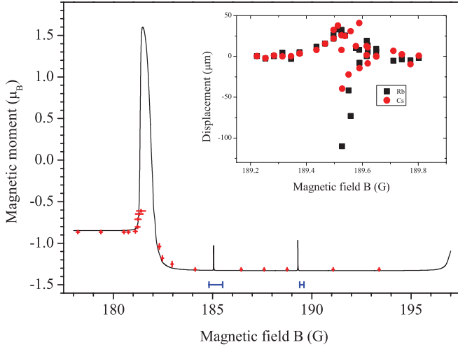
FIG. 6. (Color online) Calculated (solid line) and measured (red points) molecular magnetic moment along the magnetoassociation route starting at the 197.06 G Feshbach resonance. The two horizontal error bars mark the estimated field values for two weak avoided crossings, which we detect by variations in the cloud displacement at fixed gradient field; see inset. The crossings are visible here as spikes in the calculated curve and are indicated more explicitly in Figs. 5(b) and 5(c). (Inset) Cloud displacement as a function of magnetic field B near the weak avoided crossing at B = 189.50 G. The strong variation in the displacement data indicates the presence of the crossing. Similar data are obtained for the weak avoided crossing near B = 185.17 G.
