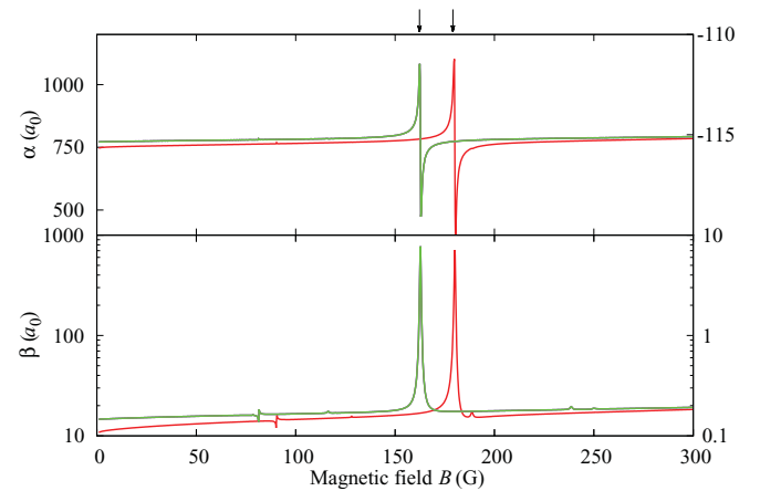
FIG. 10. (Color online) The real and imaginary parts of the complex scattering length at the Rb |2, -1\rangle + Cs |3,3\rangle threshold, calculated using the final fitted potentials: s wave (red, dark gray, left-hand axis) and p -wave (green, light gray, right-hand axis). The observed resonance positions are shown as arrows at the top of the graph. The three components of the p -wave scattering length are indistinguishable on this scale.
